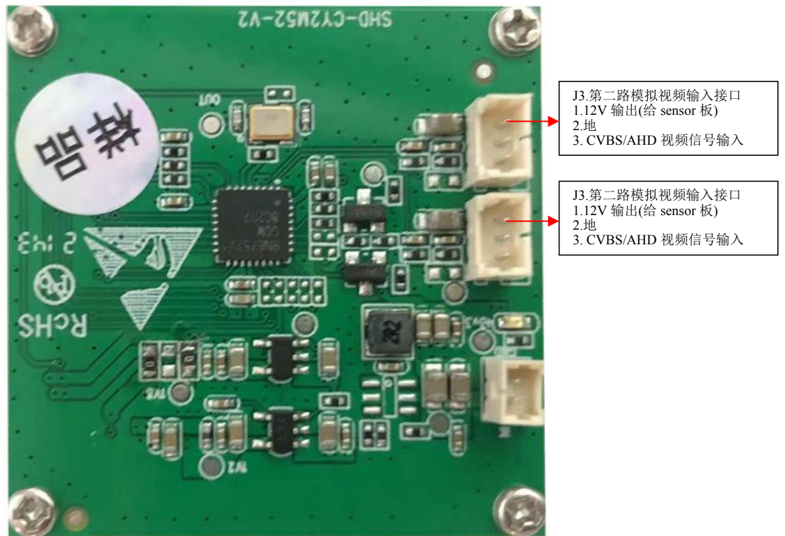
4. AHD+CVBS 接口板背面定义:
